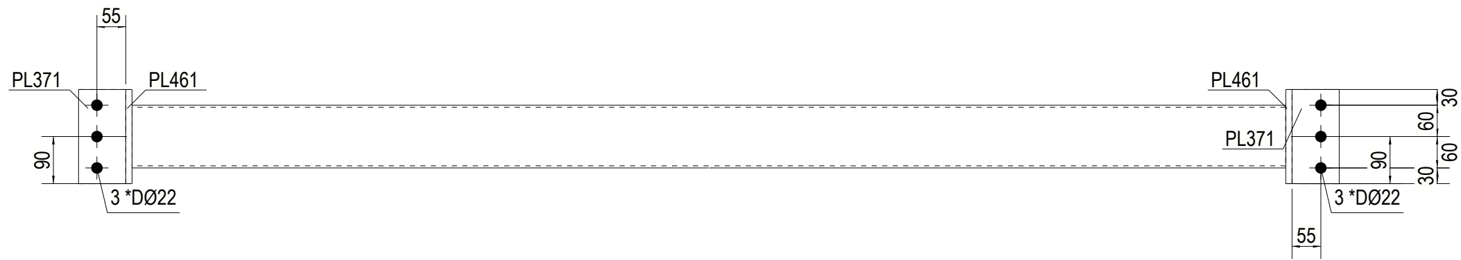
TOP VIEW
